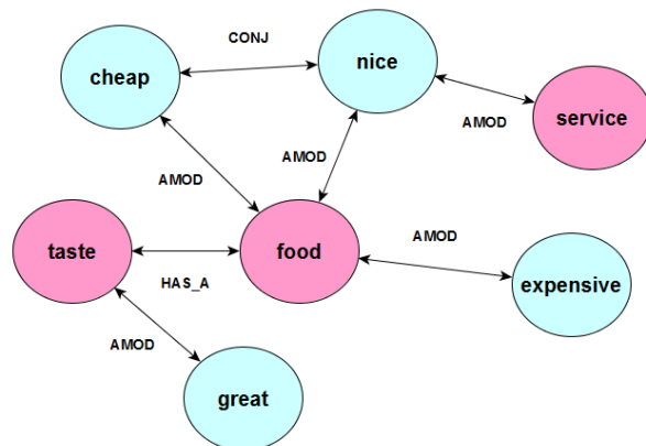
Figure 1: Example of a graph fragment constructed with the bootstrapped words and relations.
